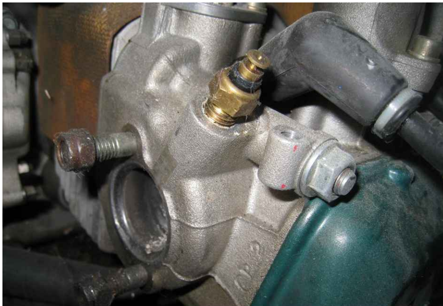
Figure 5.2: Position temperature sensor - new configuration
