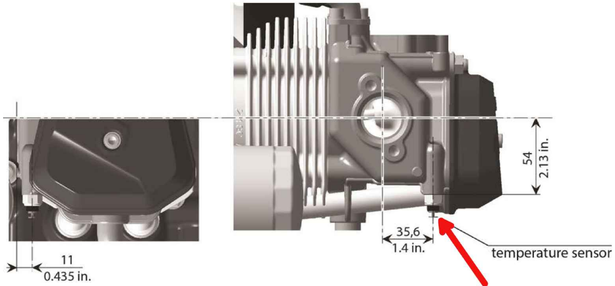
Figure 5.3: Position temperature sensor - old configuration
